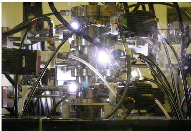
Figure 2. Modular AC/AC hybrid plasma reactor in operation (US Patent 7232975, June 2007).
